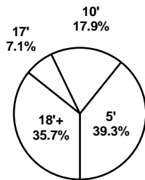
Scoring Range
