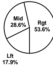
Scoring Locations
