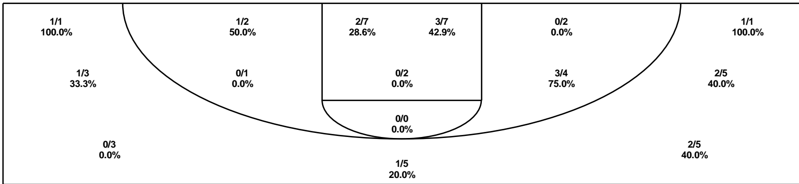
Scoring Distribution
