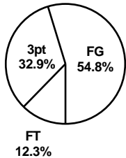
Scoring Distribution
